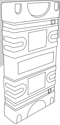
$290. MODEL# CASRMF Roto Molded Shipping Case W/ Wheels Inside Dimensions: 25"X 8"X 49" H Outside Dimensions: 27"X 10.5"X 50" H Color: Grey Weight (empty): 31 lbs.
