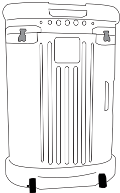
$219. MODEL# CASOVL Oval Shipping Case w/ Wheels Inside Dimensions: 21.75" X 12.5"deep X 33" H Outside Dimensions: 24" X 13"deepX34" H Color: Black Weight (empty): 26 lbs. *Can be used for shipping most pop up displays.
