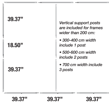
Example: Frame 97.24(h) x 118.11" (w) with one support post
